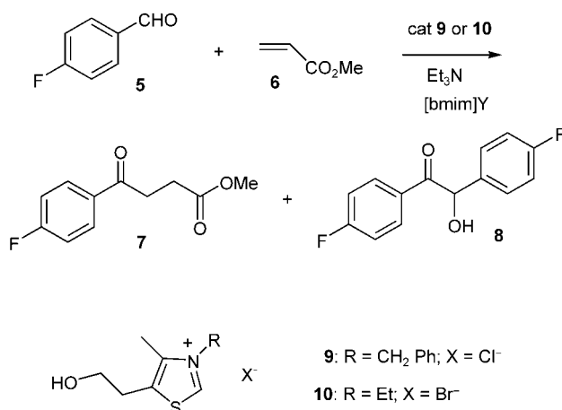
Scheme 2. Our model reaction.
