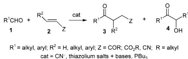
Scheme 1. The Stetter reaction.
